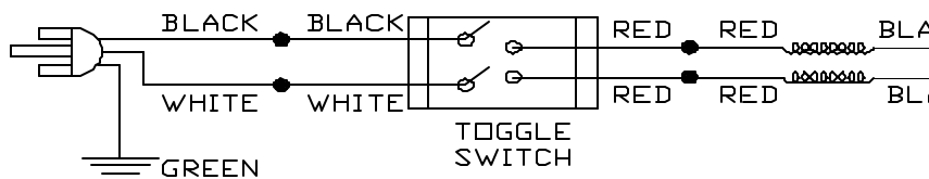
120V WIRING DIAGRAM
