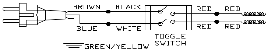
230V WIRING DIAGRAM
