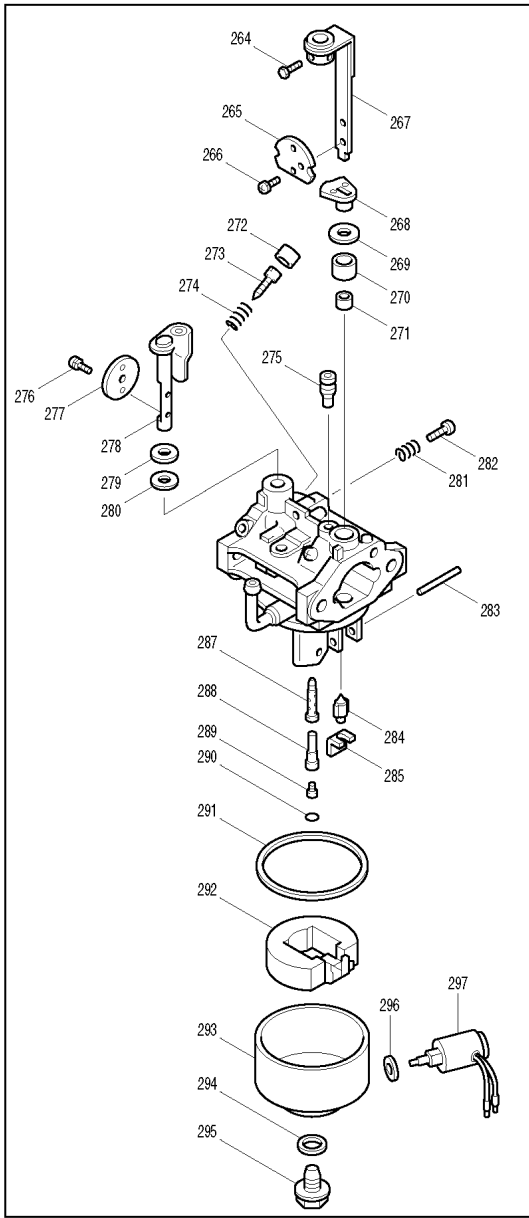
DETAIL "A"
